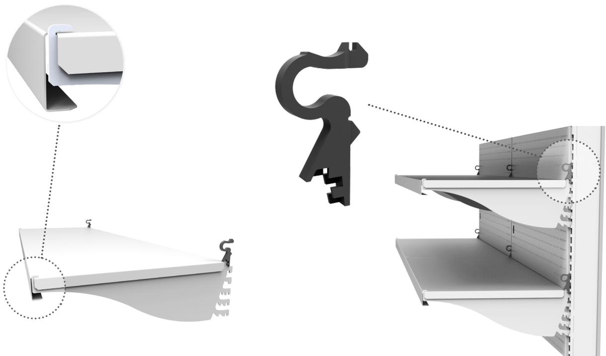
Shelf support transport lock in multidecks.
