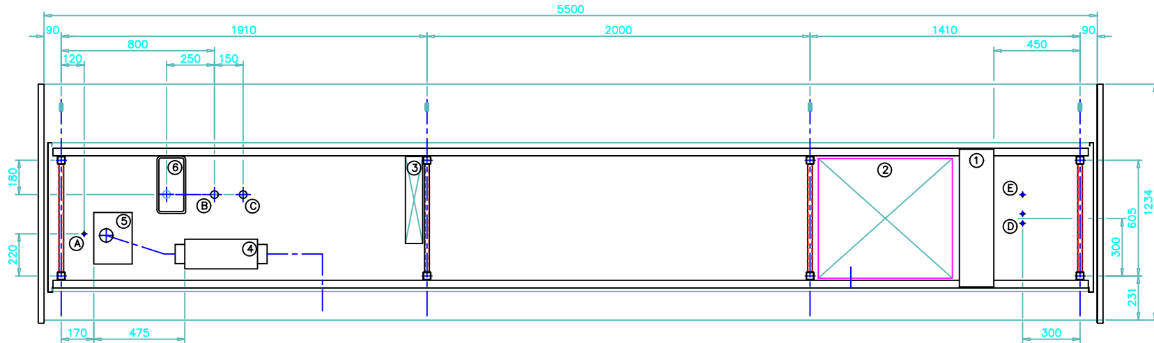
Vision 5000 Floor plan Waitrose L=5500
