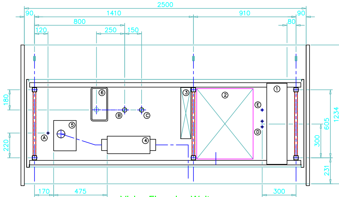
Vision Floorplan Waitrose L=2500
